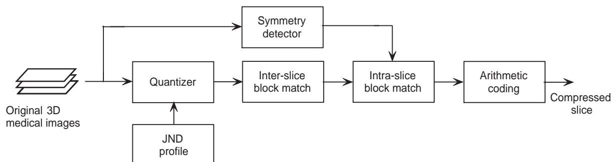
Fig. 4: Block diagram of perceptually lossless image compression with symmetry.
