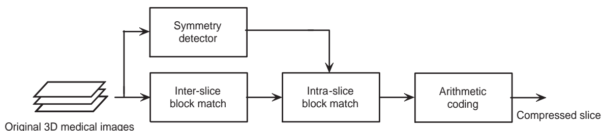
Fig. 3: Block diagram of lossless image compression with symmetry.
